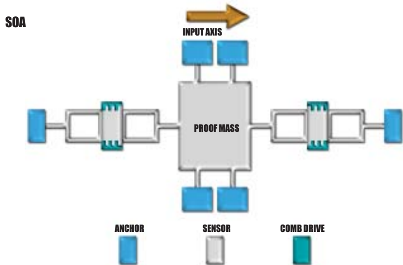
Silicon Oscillating Accelerometer (SOA) Schematic
